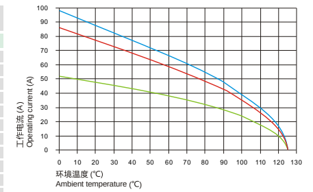
DMK70-002-F(6-16mm 2 ) DMK70-002-F(14-22mm 2 )
